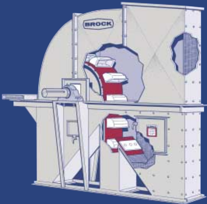
Standard Double-Trunk Head Section
