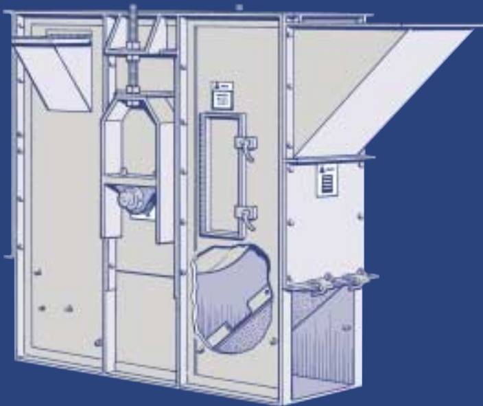
Standard Double-Trunk Boot Section
